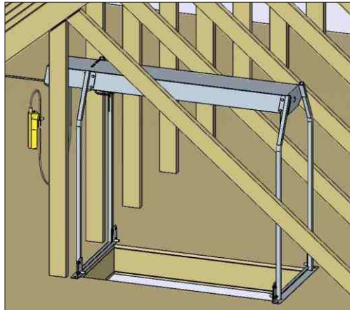
TL-24 Truss Leg Kit (only for Model 24)
